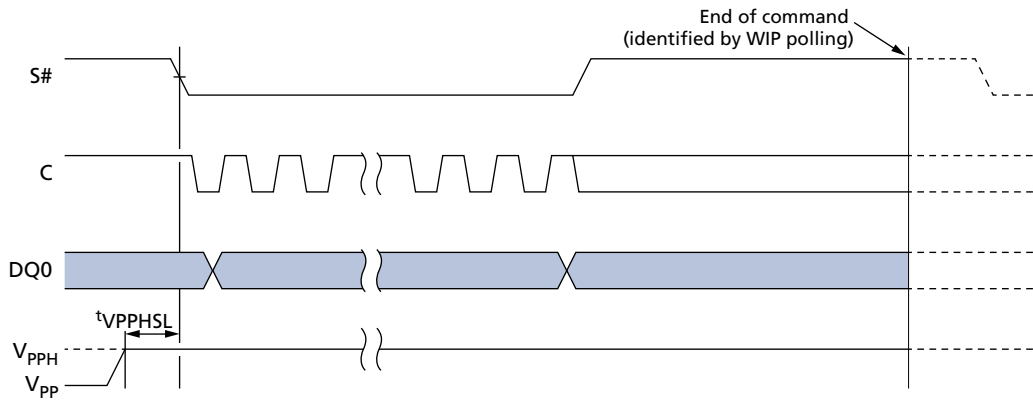
Figure 45: V_{PPH} Timing
